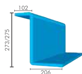
MRVC Longitudinal Beam (ICF)
