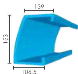
Regular Cantrail (ICF)
