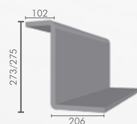
MRVC Longitudinal Beam (ICF)
