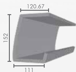
MRVC Cantrail (ICF)
